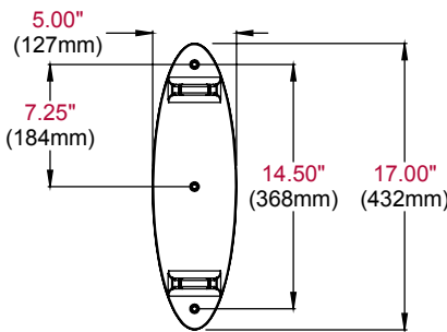
WALL PLATE
