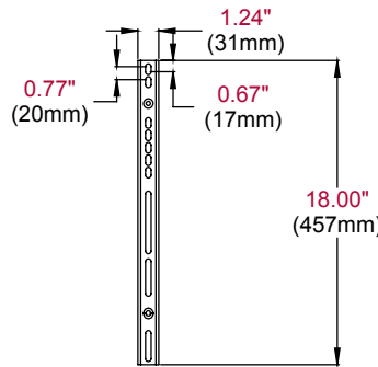
VERTICAL ADAPTER
