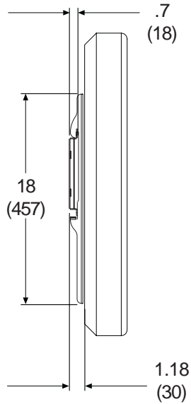
SIDE VIEW WITH SHALLOW BRACKET
