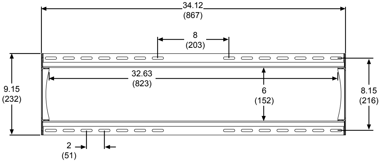
Wall Plate Detail
